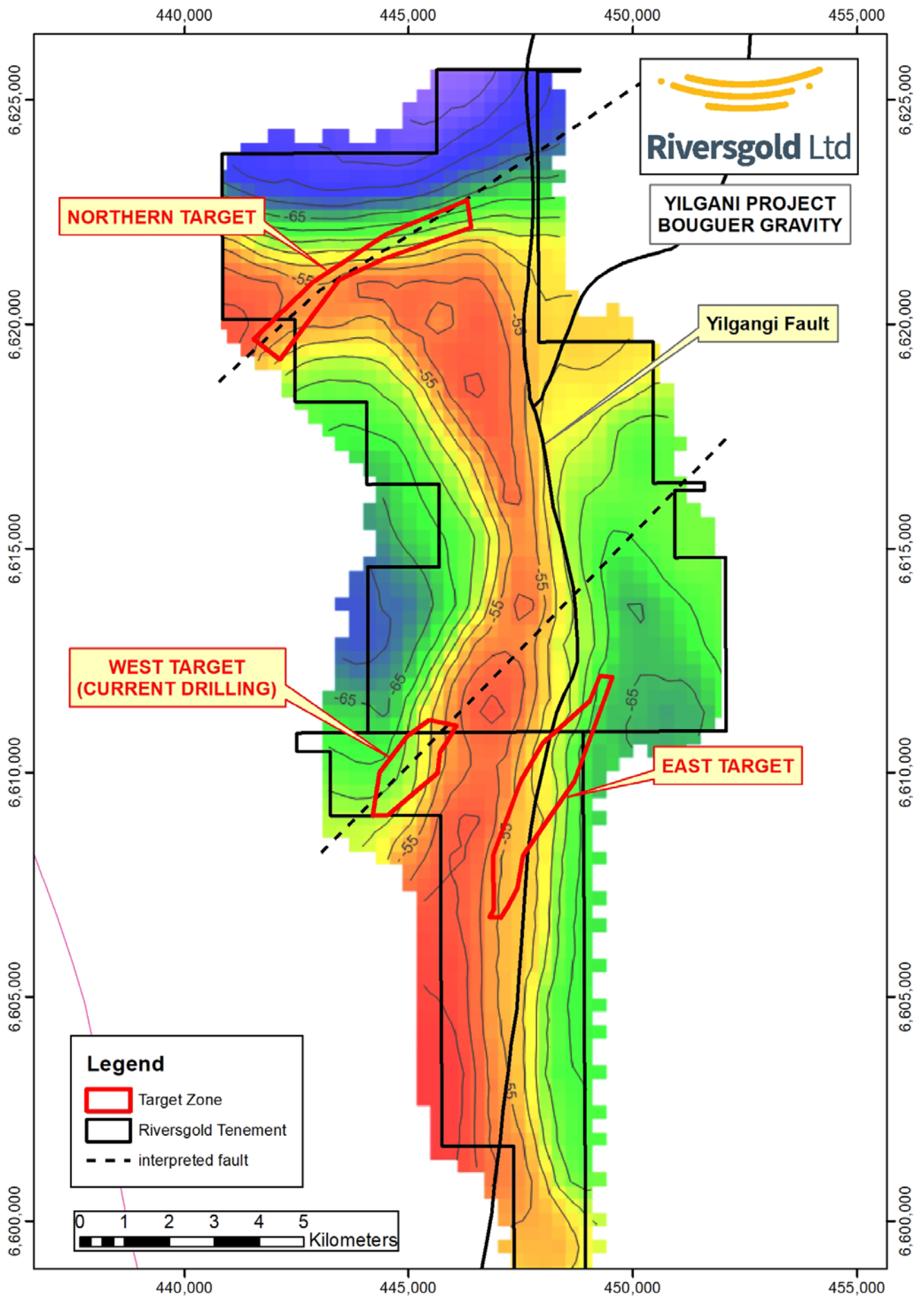
Figure 2. Yilgani Project showing bouguer gravity image with respect to drill targets (contour interval is 2mgal).
