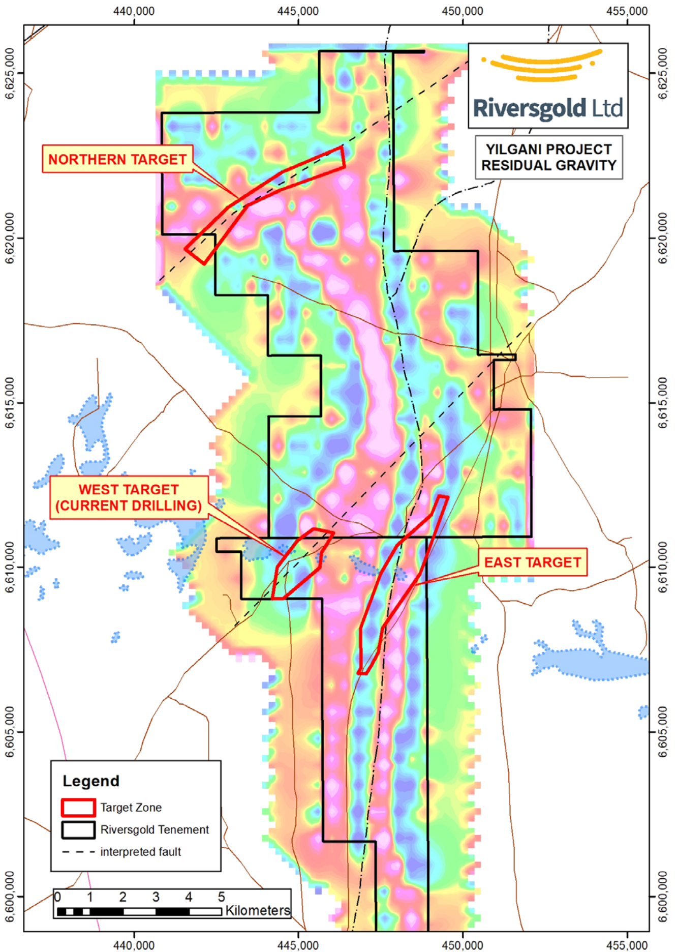
Figure 1. Yilgani Project showing residual gravity image with respect to drill targets.
